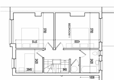
ATTIC FLOOR PLAN 1:50
